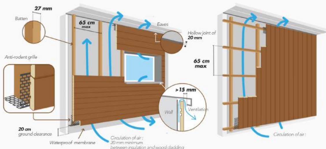
Horizontal installation
